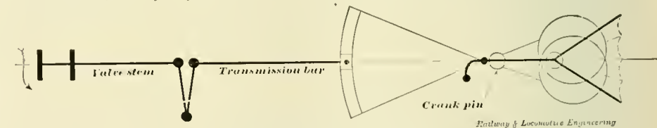
OUTSIDE ADMISSION—DIRECT.
